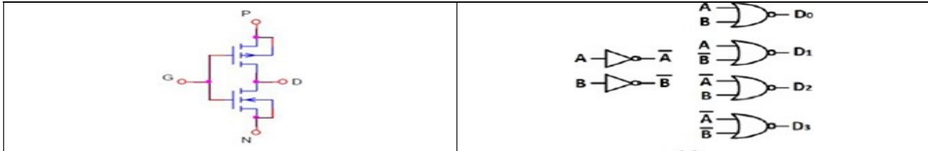
Fig 1: Basic GDI cell
