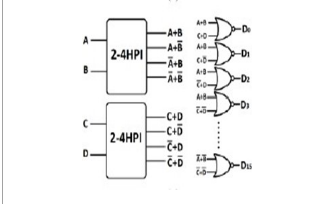
Fig 5: 4-16 mixed logic decoder
