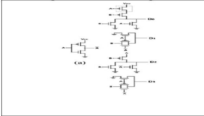
Fig 3: Mixed logic HP topology 2-4 decoder
