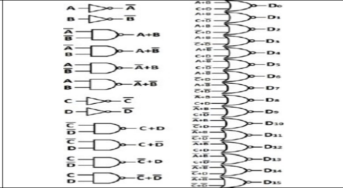
Fig 4: 4-16 CMOS decoder.
